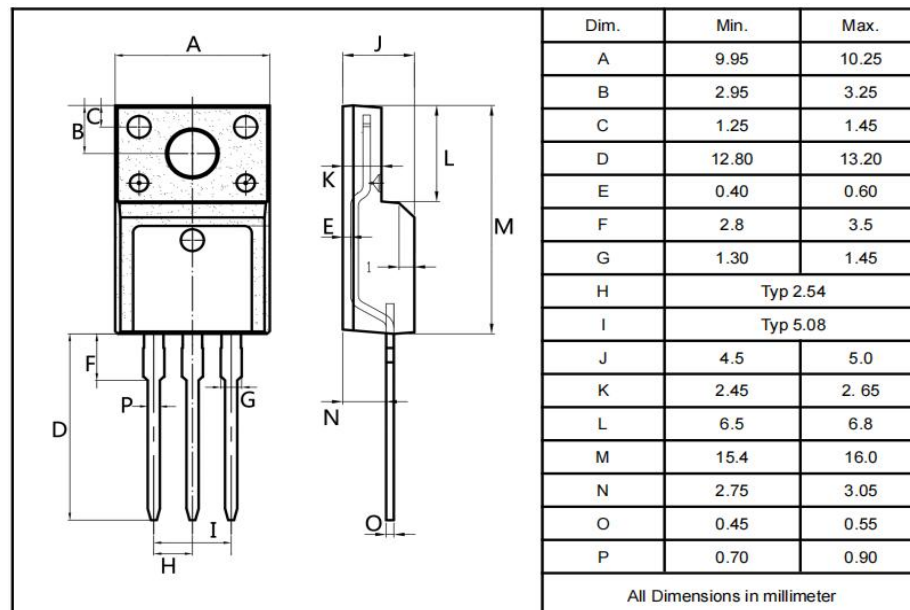
TO-220F
