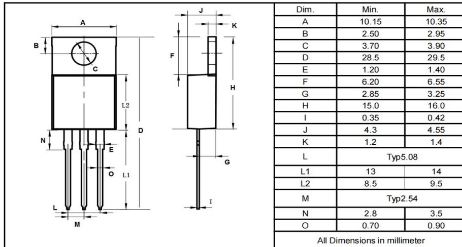
TO-220AB
